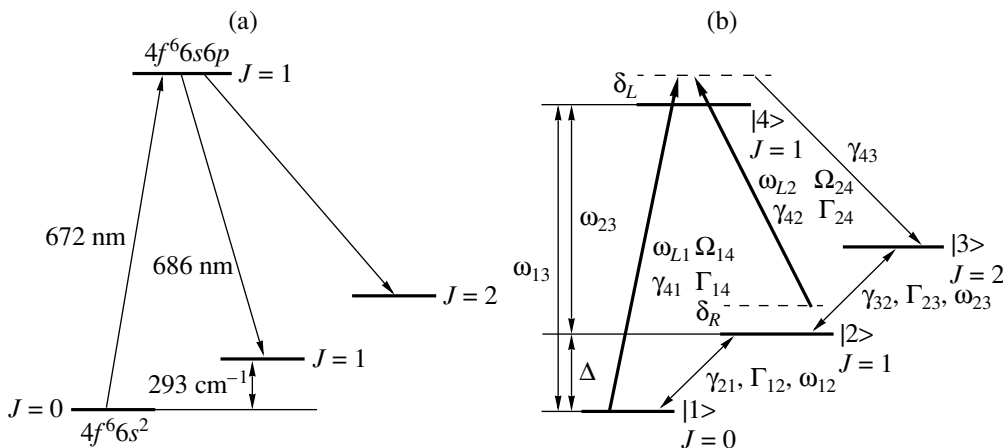
Fig. 2. (a) Diagram of energy levels of the samarium atom and (b) parameters used in calculations. The parameters are the same as in Fig. 1.
