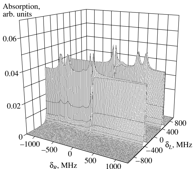
Fig. 6. Dependence of the absorption coefficient of the samarium atom at rest on \delta_R and \delta_L in applied longitudinal magnetic field.
