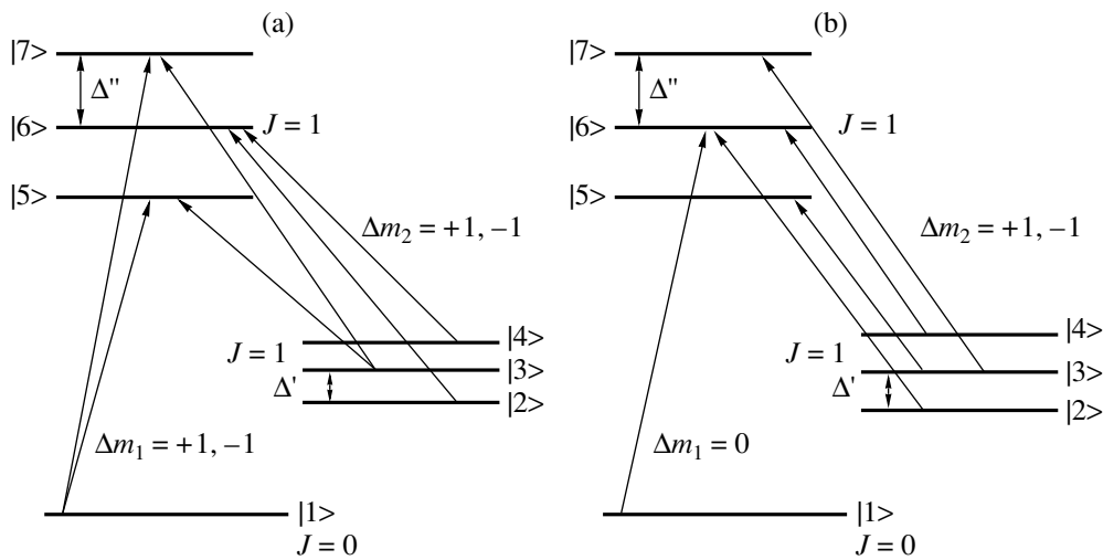
Fig. 5. Scheme of the \Lambda system of samarium atom under applied (a) longitudinal magnetic field for linear orthogonal laser beam polarizations and (b) transverse magnetic field; the selection rules for the first field are =\pm 1 = (a) \pm 1 and (b) 0; for the second field, \omega_{L2} - \Delta m_2 = \pm 1 ; \Delta' and \Delta'' are the Zeeman splittings of the upper and lower levels with J \neq 0 , respectively.
