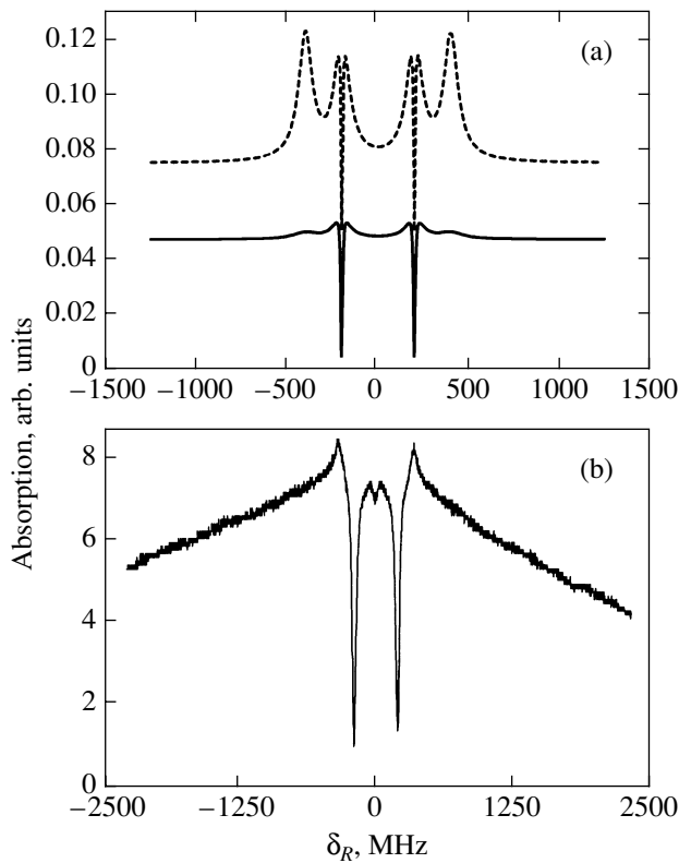
Fig. 8. (a) Theoretical dependences of the absorption coefficient of a seven-level system on Raman detuning \delta_R in a transverse magnetic field calculated taking into account the Doppler effect at T = 873 K for two magnetic sublevel depolarization values, G = 0 (solid line) and G = 0.5 (dashed line) and (b) experimental dependence of the absorption coefficient in a 29 Oe transverse field at a 0.2 torr buffer gas (Ar) pressure.
