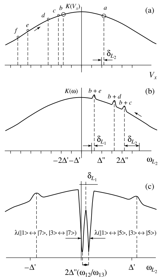
Fig. 9. Observation of coherent population trapping resonances against the background of a Doppler-broadened line; point a corresponds to the |1\rangle \leftrightarrow |7\rangle transition; b , to |1\rangle \leftrightarrow |5\rangle ; c , to |3\rangle \leftrightarrow |7\rangle ; d , to |2\rangle \leftrightarrow |6\rangle ; e , to |4\rangle \leftrightarrow |6\rangle ; and f , to the |3\rangle \leftrightarrow |5\rangle transition. (a) F(v_x) is the Maxwell velocity distribution function, points a and b correspond to particles with a definite velocity projection onto the beam propagation direction, namely, the projection at which the Doppler shift balances the detuning of field \omega_{L1} from the |1\rangle \leftrightarrow |7\rangle and |1\rangle \leftrightarrow |5\rangle quantum transition frequencies, respectively; points c , d , e , and f correspond to the velocity groups of particles for which the Doppler shift balances detuning \delta_{L2} of frequency \omega_{L2} from the |3\rangle \leftrightarrow |7\rangle , |2\rangle \leftrightarrow |6\rangle , |4\rangle \leftrightarrow |6\rangle , and |3\rangle \leftrightarrow |5\rangle quantum transition frequencies, respectively; (b) illustration of the formation of absorption peaks; and (c) illustration of the formation of coherent population trapping resonances against the background of a Doppler-broadened line.
